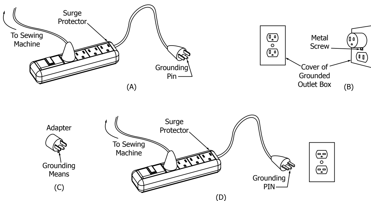
Grounding Methods Figure 61.1
